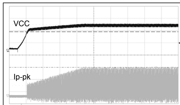
Figure 9 Soft Start
