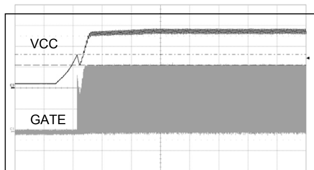
Figure 8 Start-up
